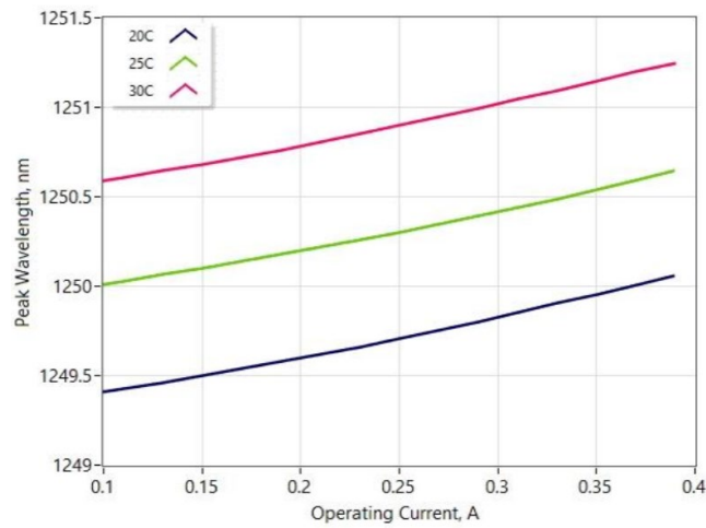
Peak Wavelength Tuning by Current
